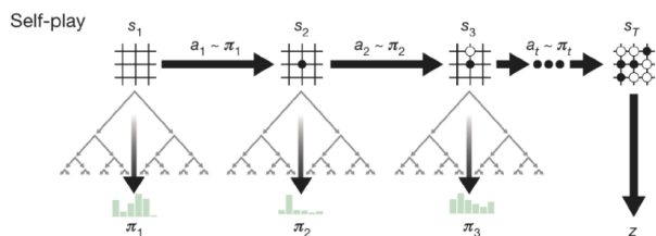
图3 Self-play 过程示意图 Fig.3 Self-play process diagram
